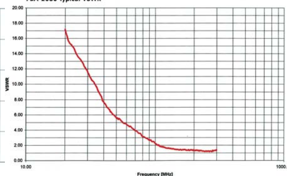
PBA-2030 Typical VSWR
